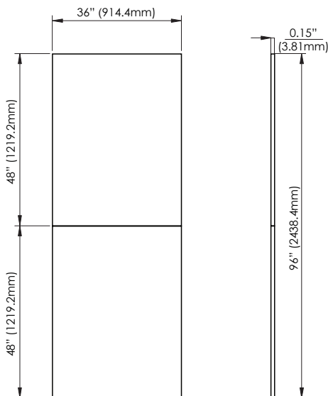
SIDE WALL
