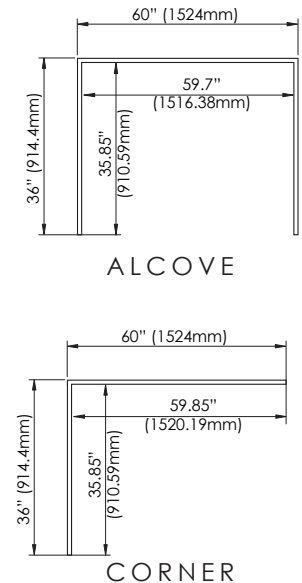
TOP VIEW (ASSEMBLED)
