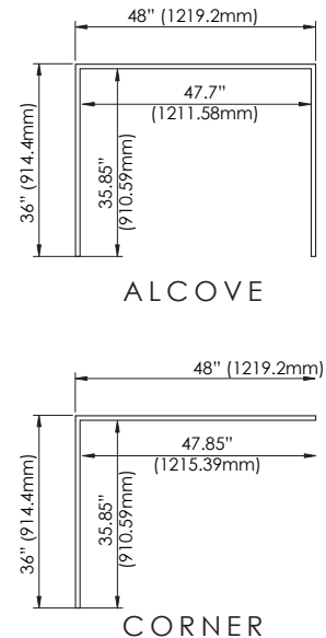
TOP VIEW (ASSEMBLED)
